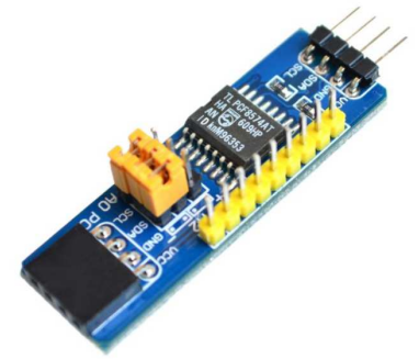
[2511] Tarjeta De Expansi3n Pcf8574 Expansion Board I2c Arduino
