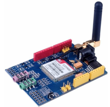
[2231]Modulo Gsm Shield SIM900A Module Quad-Band GSM/GPRS
