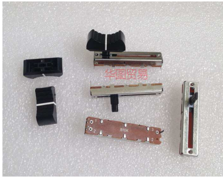
[1866]Potenciometro Deslizable 10k Lineal 45mm B10k SL-302N
