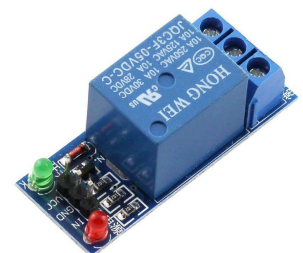
[5657]Modulo Rele Biestable Flip-flop 12v Salida Relay
