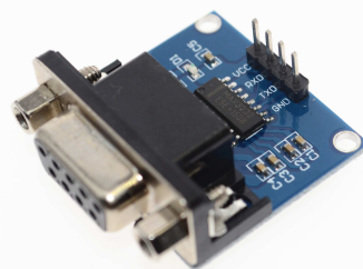
[1553]Modulo Conector Max3232 Rs232 Serial Port Ttl Converter Db9
