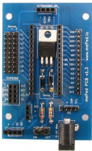
[2559]Modulo Shield Arduino Nano Littlebots Control Board
