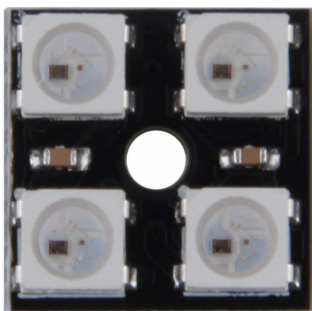
[1972]Modulo Led Rgb Inteligente Ws2812b CJMCU2816 2x2 4 bit
