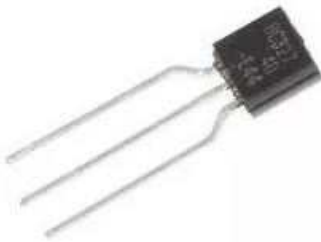
[2021x10]10 X Transistor Pnp Bc327-40 5v 500ma To-92 327 Bc327
